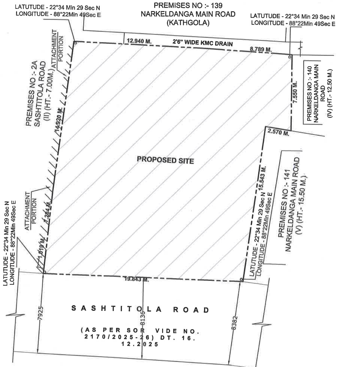
LOCATION PLAN WITH CO-ORDINATES SCALE-1:200
